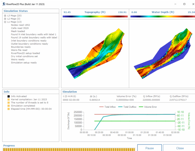
RiverFlow2D output graphics.
