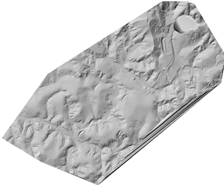
Digital elevation model with Hillshade render.
