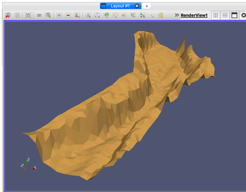
Figure 21.17 – Alternative 3D bed elevation representation.
