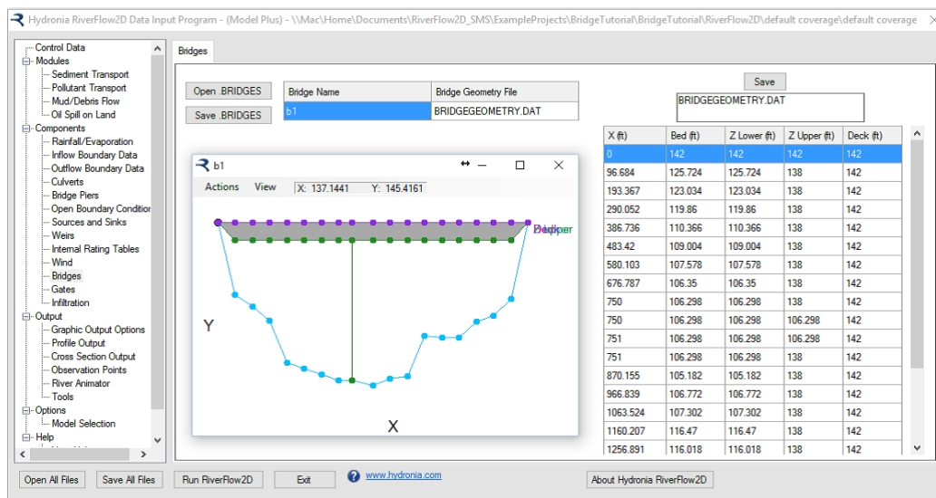
Figure 5.4 – Bridges panel.
