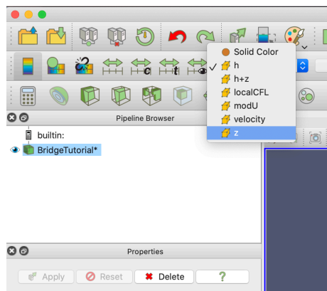
Figure 21.5 – Variable selector.
