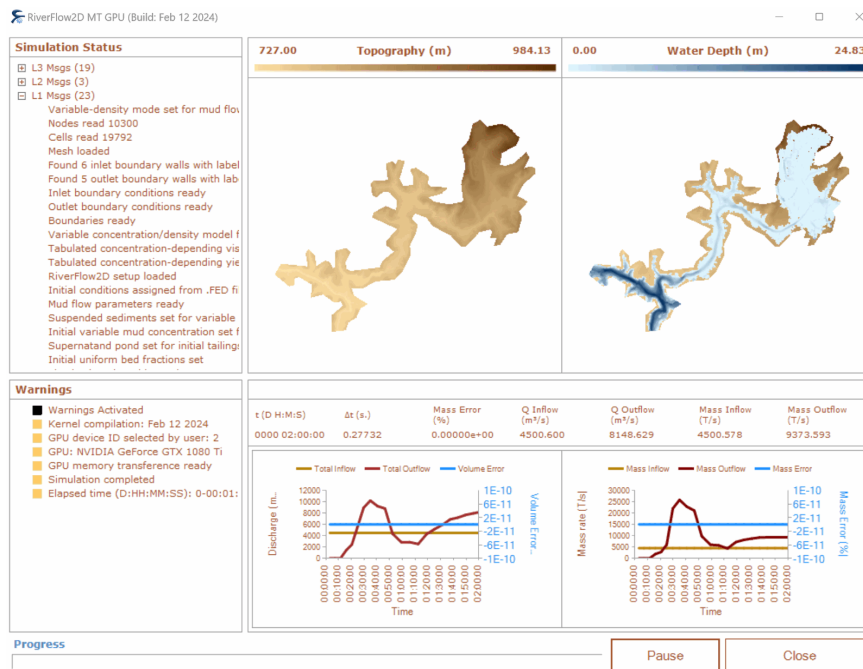
RiverFlow2D model execution window.
