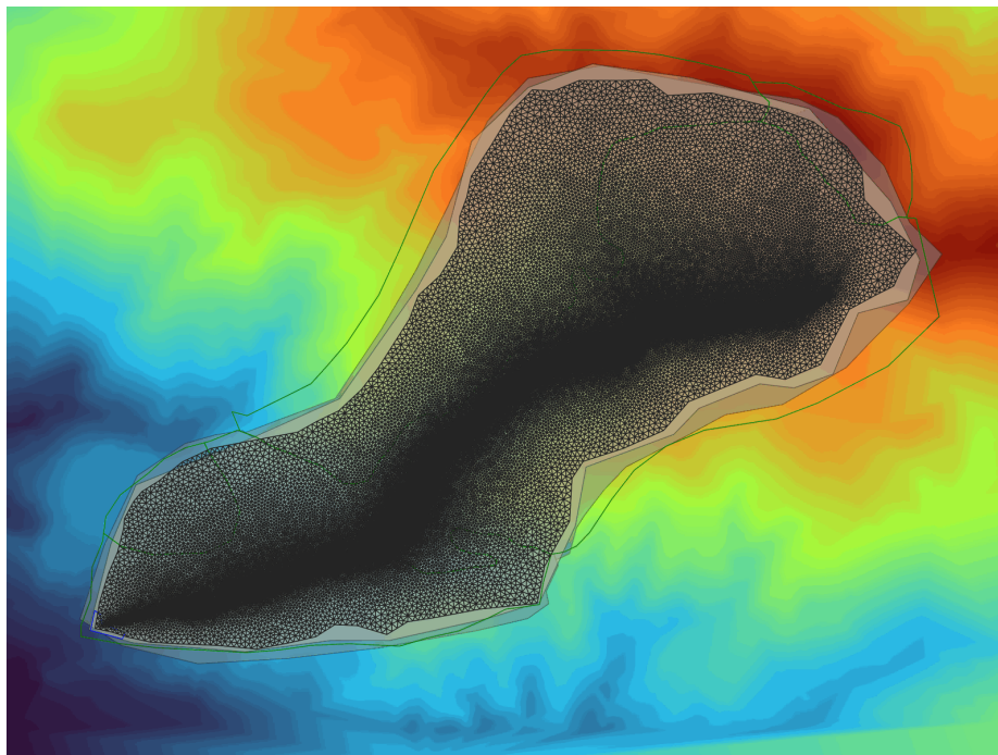
Figure 11.2 – Final mesh.
