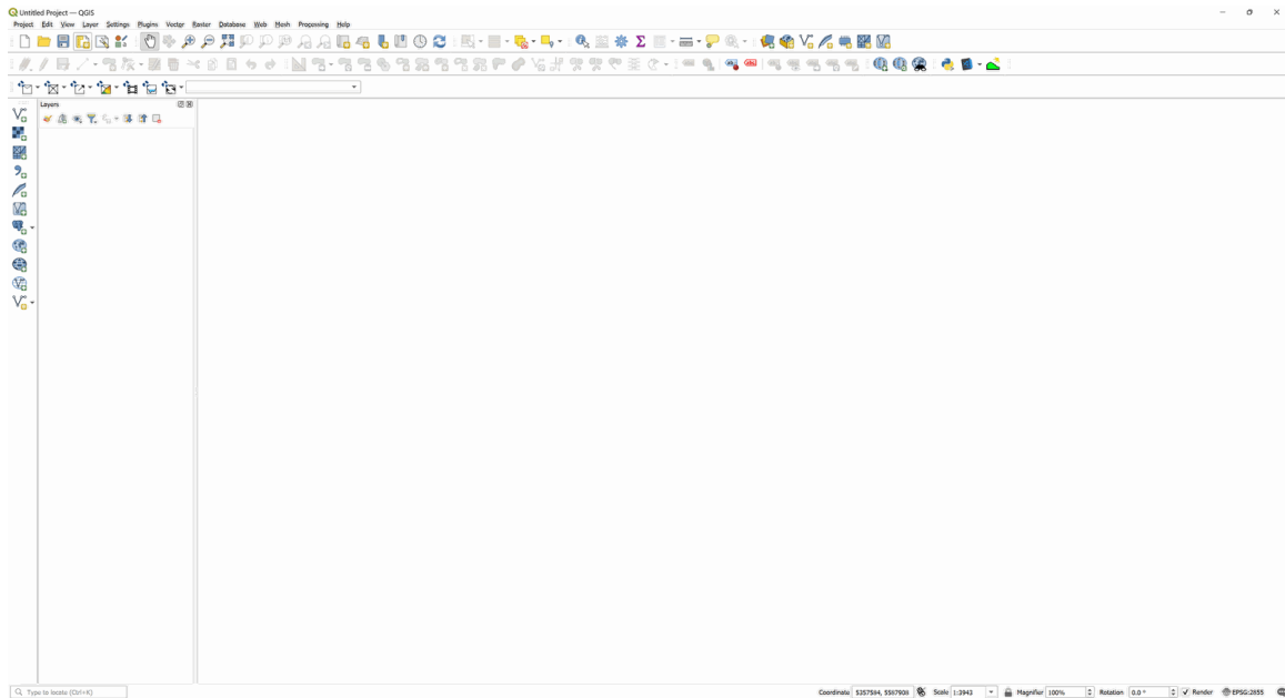
Figure 12.4 – QGIS interface.
