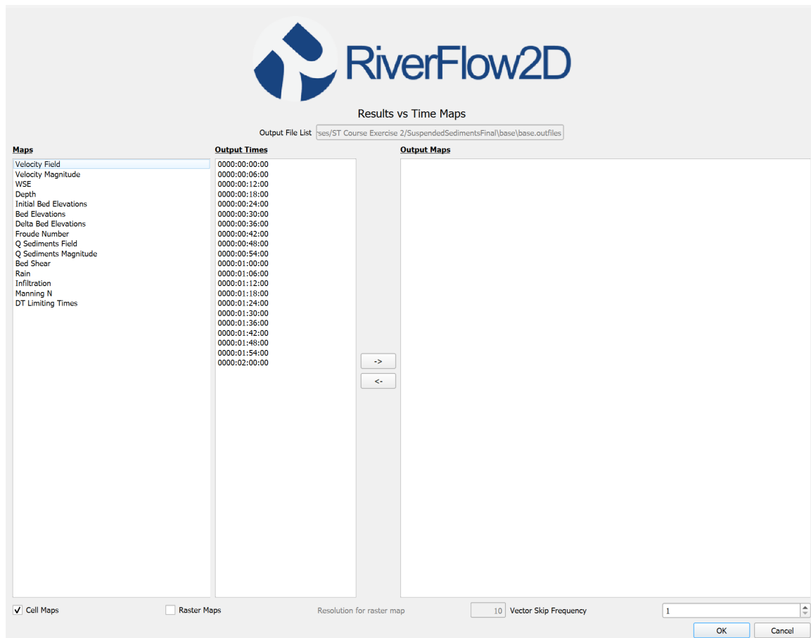
Figure 4.3 – Results vs Time Maps Dialog for RiverFlow2D
