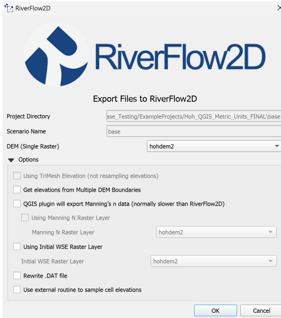
Figure 3.2 – Export Files to RiverFlow2D Dialog.
