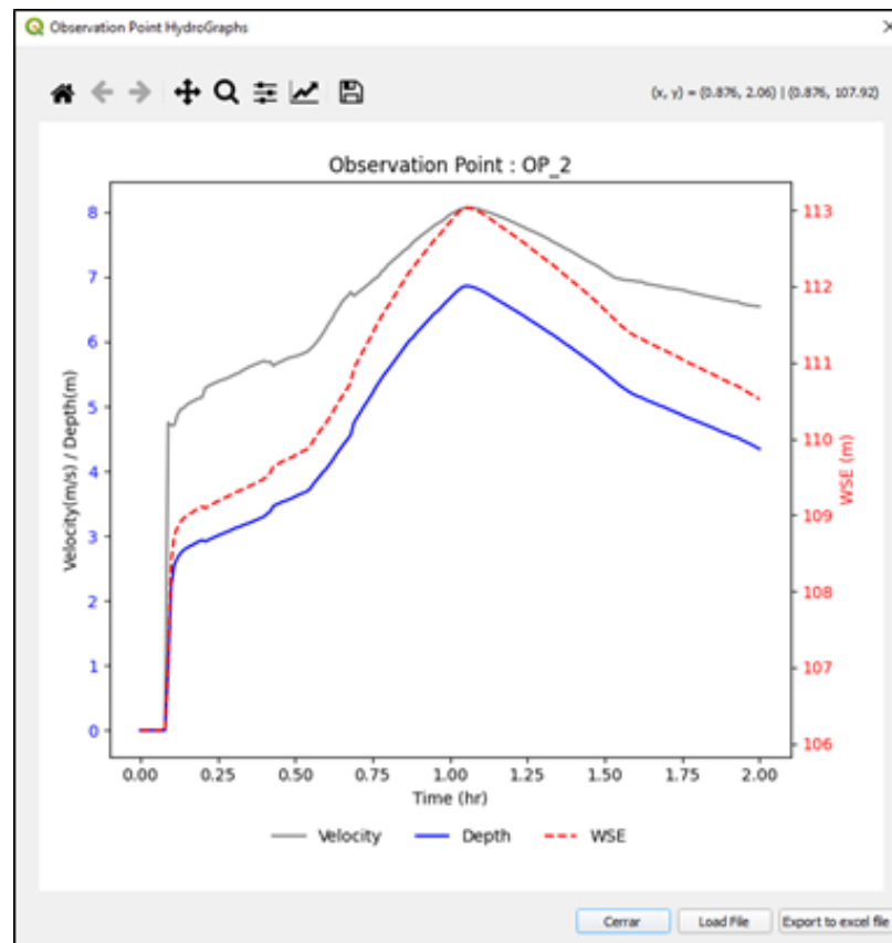
Figure 8.19 – ObservationPoint HydroGraphs
